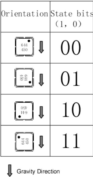
FIGURE 3-1 Device Orientation
