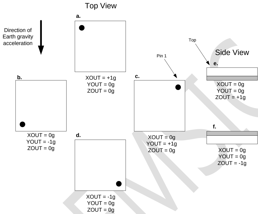
Figure 3. Package Orientation
